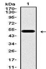
Western blot analysis of human (AA: 39-2...
