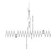
Chemical Structure (132172-61-3)
