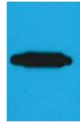
Western blot analysis of recombinant RFP...
