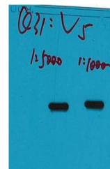
Western blot analysis of V5 recombinant
