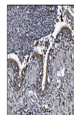
IHC analysis of KCNQ2 using anti-KCNQ2 a...
