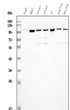
Western blot analysis of KCNQ2 using ant...
