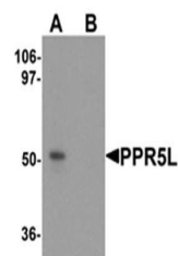
Western blot analysis of 3T3 cell lysate...
