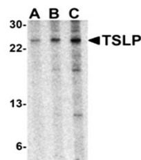
Western blot analysis of A-20 cell lysat...
