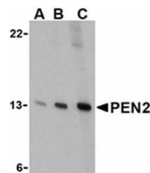
Western blot analysis of K562 cell lysat...
