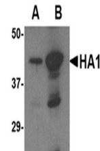
Western blot analysis of (A) 5 ng and (B...
