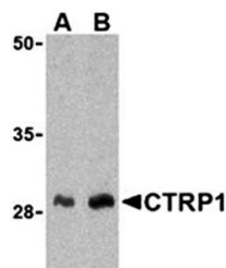
Western blot analysis of human kidney ce...
