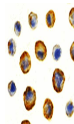
3) and THP-1 (2
