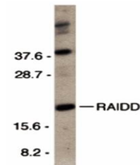
Western blot analysis of HeLa total cell...
