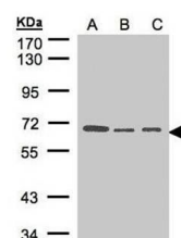
Western Blot analysis of A:293T, B:H1299...
