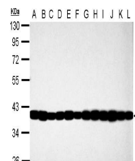
Western Blot analysis of A:Jurkat, B:Raji...
