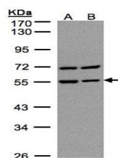
Western Blot analysis of A:MOLT4, B:Raji...
