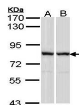
Western Blot analysis of A:A431, B:Raji ...
