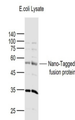
Western blot: Lane 1: Nano-Tagged Fusion P...
