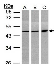
Western Blot analysis of A:293T, B:MOLT4...
