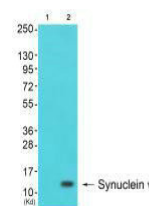
Western blot analysis of cos-7 cells (La...
