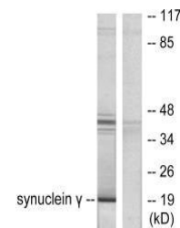
Western blot analysis of HT29 cells usin...
