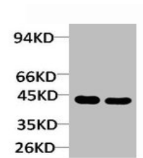
Western blot analysis of 1) Rat LiverTis...
