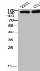
Western blot analysis of 293T(Lane 1), C...
