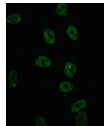
Immunofluorescent analysis of hnRNP A/B expression.
