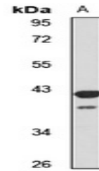
Western blot analysis of hnRNP A/B expression.
