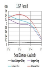
Line graph illustrates about the Ag-Ab r...
