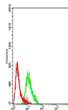
Flow cytometric analysis of SK-N-SH cell...
