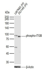
Western blot: Lane 1: Human U87MG cell; Lan...
