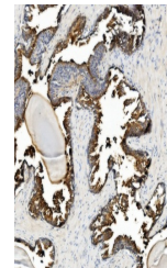
IHC analysis of ANPEP using anti-ANPEP a...
