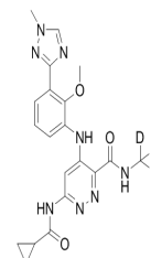
Chemical structure of Tyk2-IN-4 (BMS9861...)
