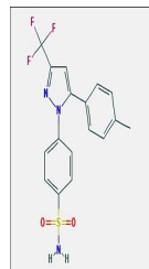
Chemical structure of Celecoxib
