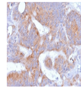
IHC testing of FFPE human colon with rec...
