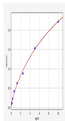
Human PARP4(Poly ADP Ribose Polymerase 4...
