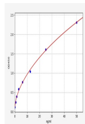
Human RSAD2(Radical S-adenosyl methionin...
