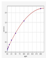
Human GLS(Glutaminase kidney isoform, mi...
