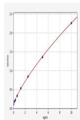
Human GUCY2C(Heat- stable enterotoxin rec...
