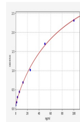
Bovine IFI30(Gamma-interferon-inducible ...
