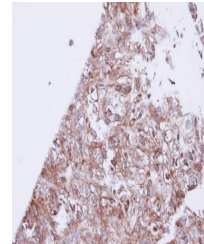
Immunohistochemical staining of DU145 cells.
