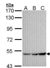
Western blot analysis of A431 (Lane 1), H...
