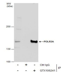
Immunoprecipitation analysis of SK-N-SH
