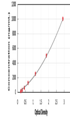
Standard Curve of Bovine Haptoglobin ELISA
