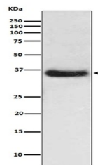
WB analysis of IKB alpha expression in H...
