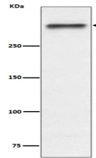
WB analysis of 53BP1 expression in HeLa ...
