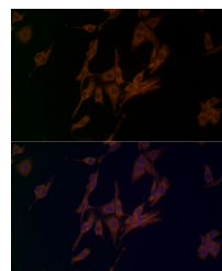
Immunofluorescence analysis of PC-12 cells
