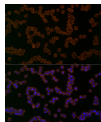
Immunofluorescence analysis of K-562 cells
