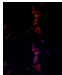
Immunofluorescence analysis of SH-SY5Y cells
