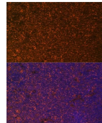
Immunofluorescence analysis of rat breast tissue
