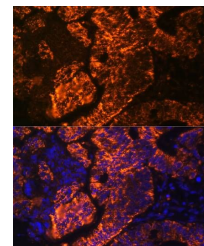
Immunofluorescence analysis of human colon tissue
