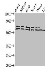
Western blot analysis of MCF-7 (lane 1), ...
