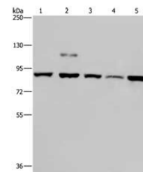
Western blot aanalysis of Lane 1-5: Jurk...
