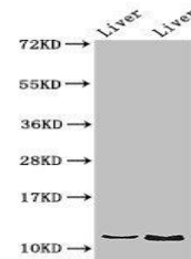
Western blot analysis of Rat liver(lane ...
