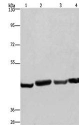
Western blot analysis of Lane 1-4: A549...
