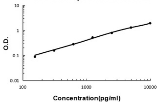
Mouse Cathepsin B PicoKine ELISA Kit standard curve
