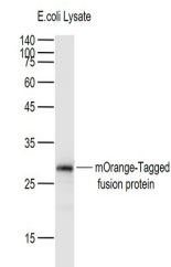
Western blot: Lane 1: mOrange-Tagged fusion protein
