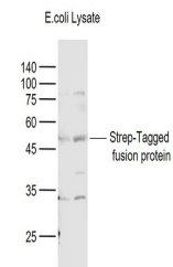
Western blot: Lane 1: Strep-Tagged Fusion ...
