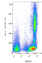
Flow cytometry analysis (surface stainin...
