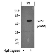
Western blot analysis of Cdc25B(Phospho- ... ...
