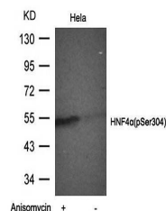
Western blot analysis of HNF4 \alpha (Phospho-Ser304)
